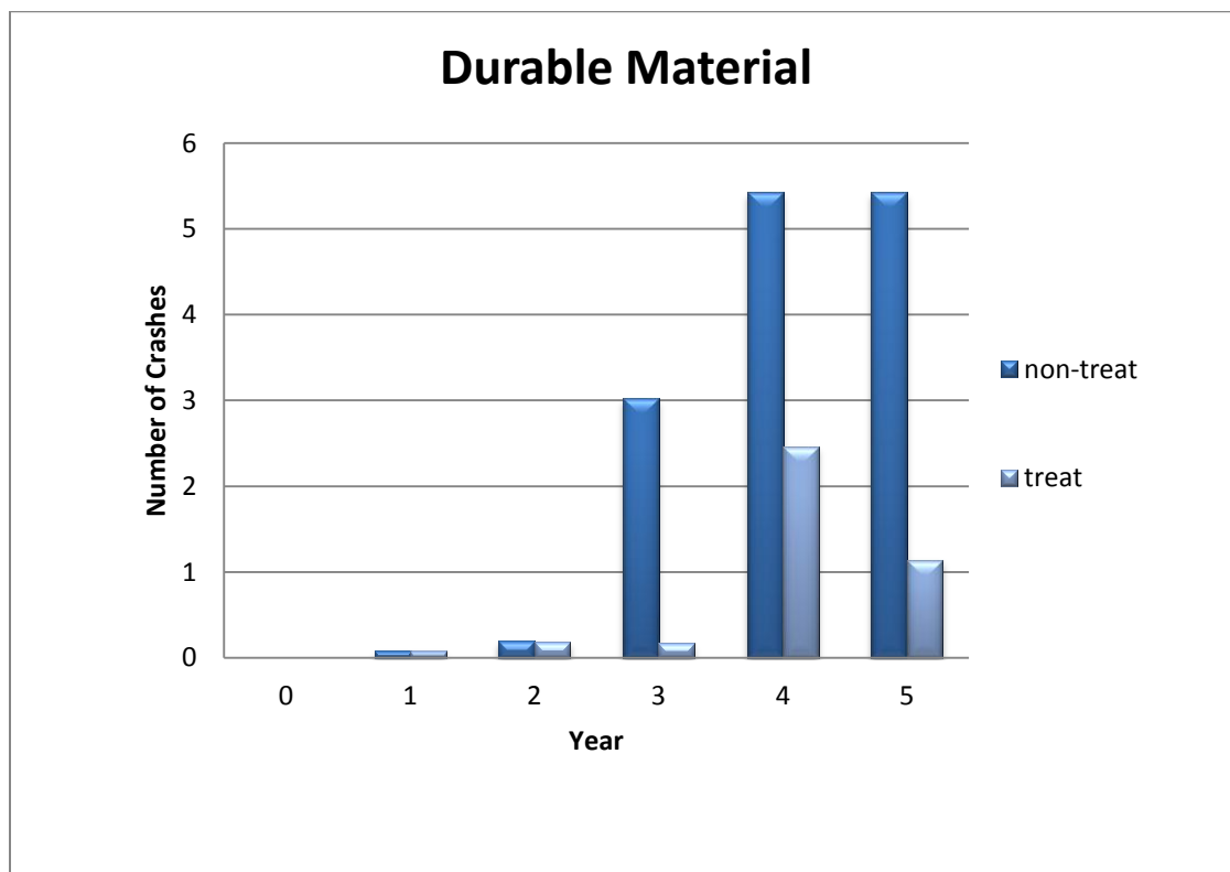
Figure B.35. Durable marking NPV in Range 6
