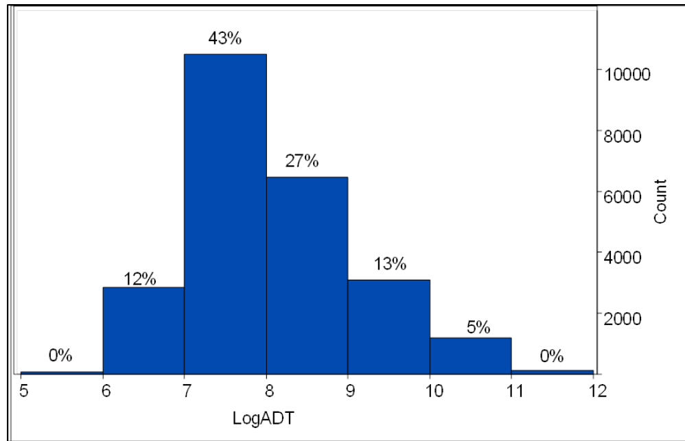
Figure 6.4. Histogram of \log(\text{ADT})
