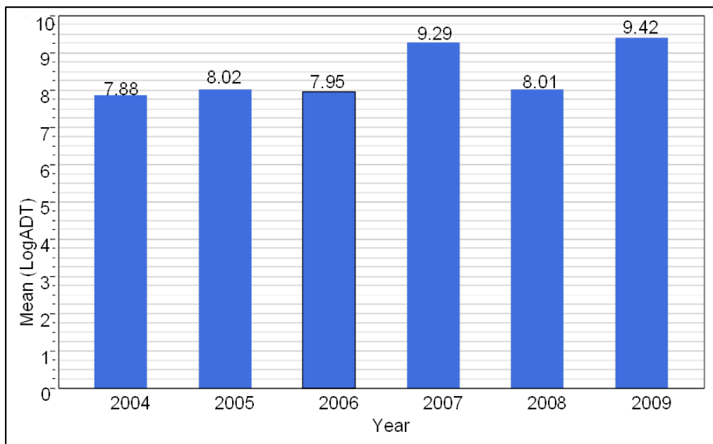
Figure 6.5. Distribution of \log(\text{ADT}) by year
