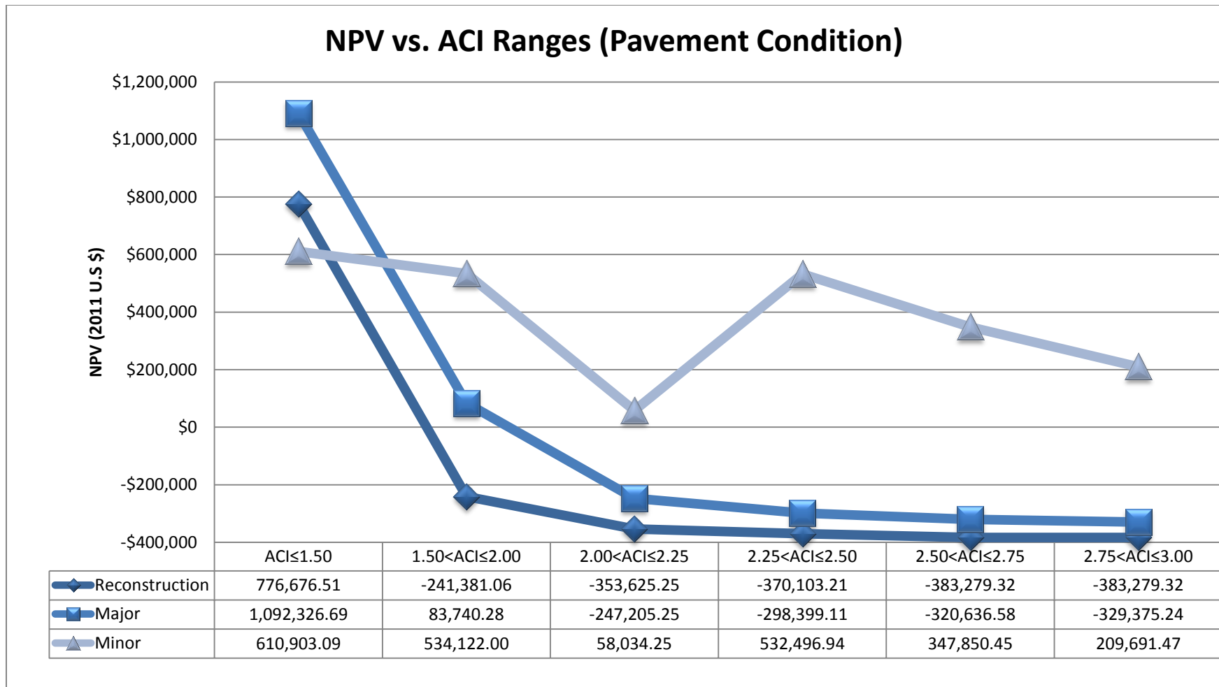
Figure 7.2. NPV for pavement condition group alternatives by ACI range
