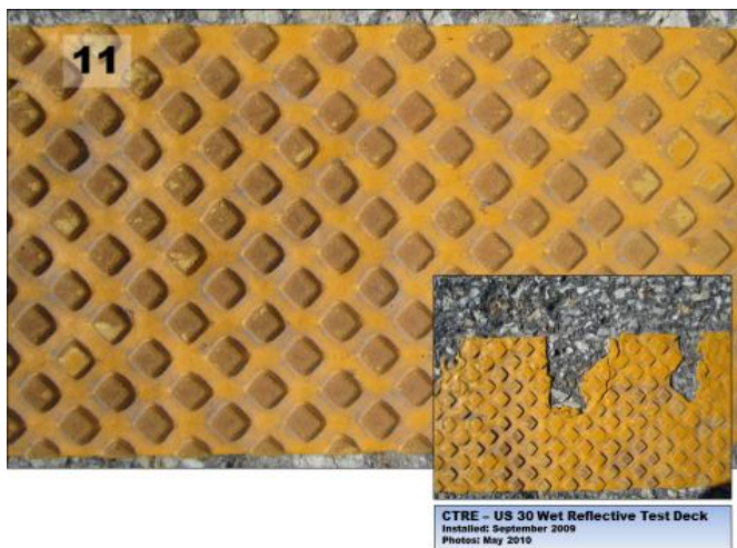
Figure 9. 3M test sections 11 and 12 after one winter
