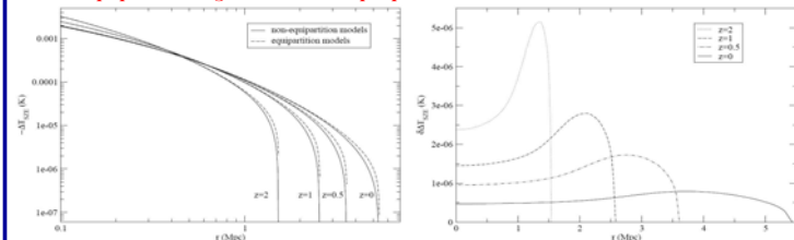
Figure 5 (left panel): SZ temperature decrement profiles, -\Delta T_{\text{SZE}} , of our simulated cluster at four different redshifts. The non-equipartition models ( \beta = 1/1800 ) are shown in solid lines while the equipartition models are shown in dashed lines.
