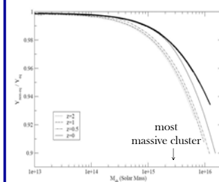
Figure 7: Integrated SZ biases, Y_{\text{non-eq}}/Y_{\text{eq}} , as a function of M_{\text{sh}} for both our simulated realistic NFW model in the \Lambda CDM Universe (thin lines) and the numerical simulated self-similar (SS) model in the Einstein-de Sitter Universe (thick lines) at four different redshifts. We assume f_{\text{gas}} = 0.17 for the SS model. The four lines for the SS model lie almost along the same line which cannot be easily distinguished on the graph.
