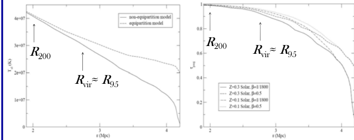
Figure 1 (left panel): Projected X-ray spectroscopic-like temperature profiles for both equipartition model and non-equipartition models. Non-adiabatic electron heating efficiency \beta = 1/1800 and metallicity Z = 0.3Z_{\odot} are assumed here.
