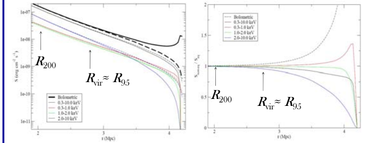
Figure 3 (left panel): Surface brightness profiles, S , for various energy bands for the non-equipartition (solid lines) and equipartition (dashed lines) cluster models at z = 0 . Models are the same as in Figure 1.
