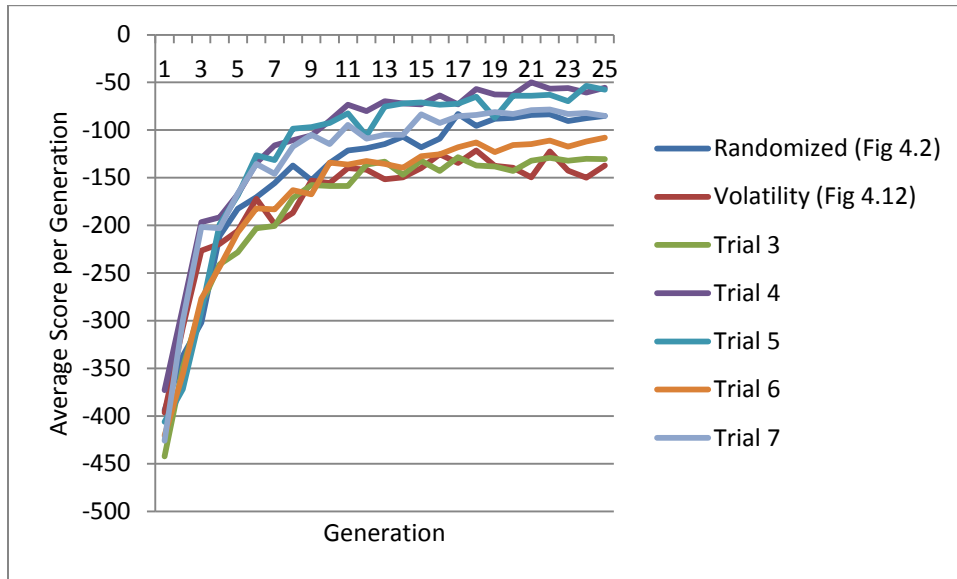
Figure 4.14: Seven GL Memory Trials with Randomized Initialization
