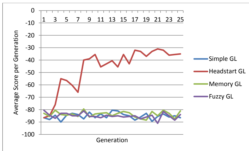
Figure 4.5: Genetic Learning Team Results of H17-Initialized Test
