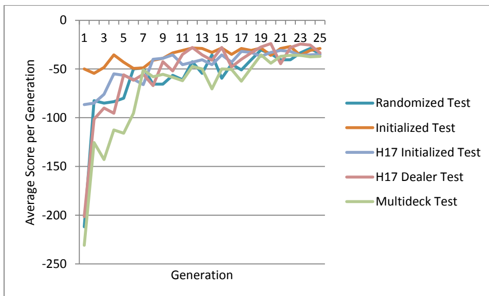
Figure 4.15: Headstart Team Progress Across Multiple Tests
