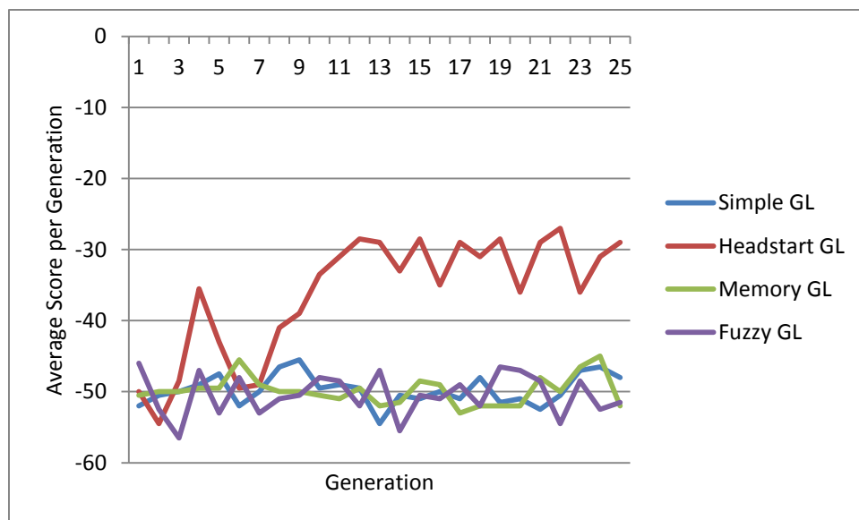
Figure 4.4: Genetic Learning Team Results of Initialized Test
